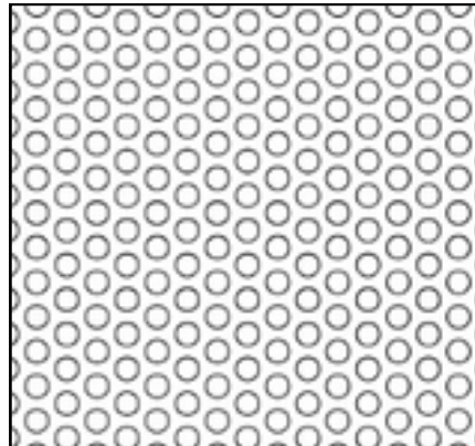
Pattern: Round Staggered Hole: 0.125" Centers: 0.188" Open Area: 40.3%
