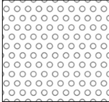
Pattern: Round Staggered Hole: 0.125" Centers: 0.250" Open Area: 22.7%
