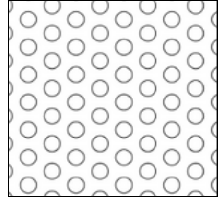
Pattern: Round Staggered Hole: 0.125" Centers: 0.219" Open Area: 29.5%
