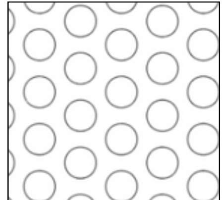
Pattern: Round Staggered Hole: 0.375" Centers: 0.562" Open Area: 40.3%
