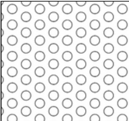
Pattern: Round Staggered Hole: 0.188" Centers: 0.313" Open Area: 32.7%
